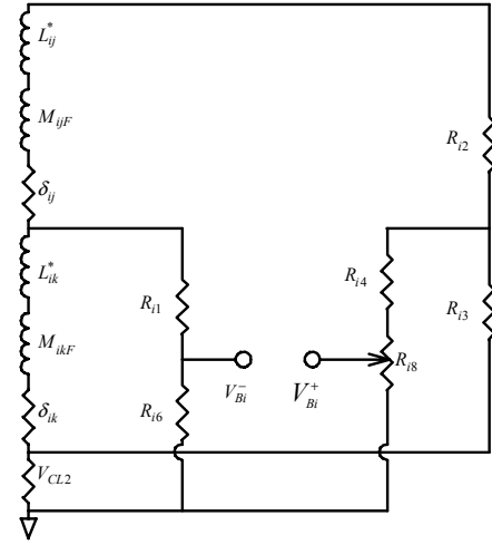
Fig. 4. Arrangement for the C-coil balance bridges.
