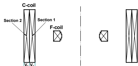
Fig. 1. Arrangement of the LDX C-coil and F-coil during inductive charging.
