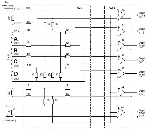
Fig. 3. Arrangement of the voltage divider designed for the C-coil.
