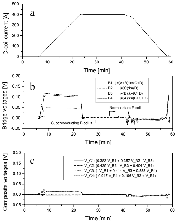
Fig. 5 a) Time variation in C-coil current, b) balance bridge voltages and c) composite bridge voltages during inductive discharge of F-coil current.
